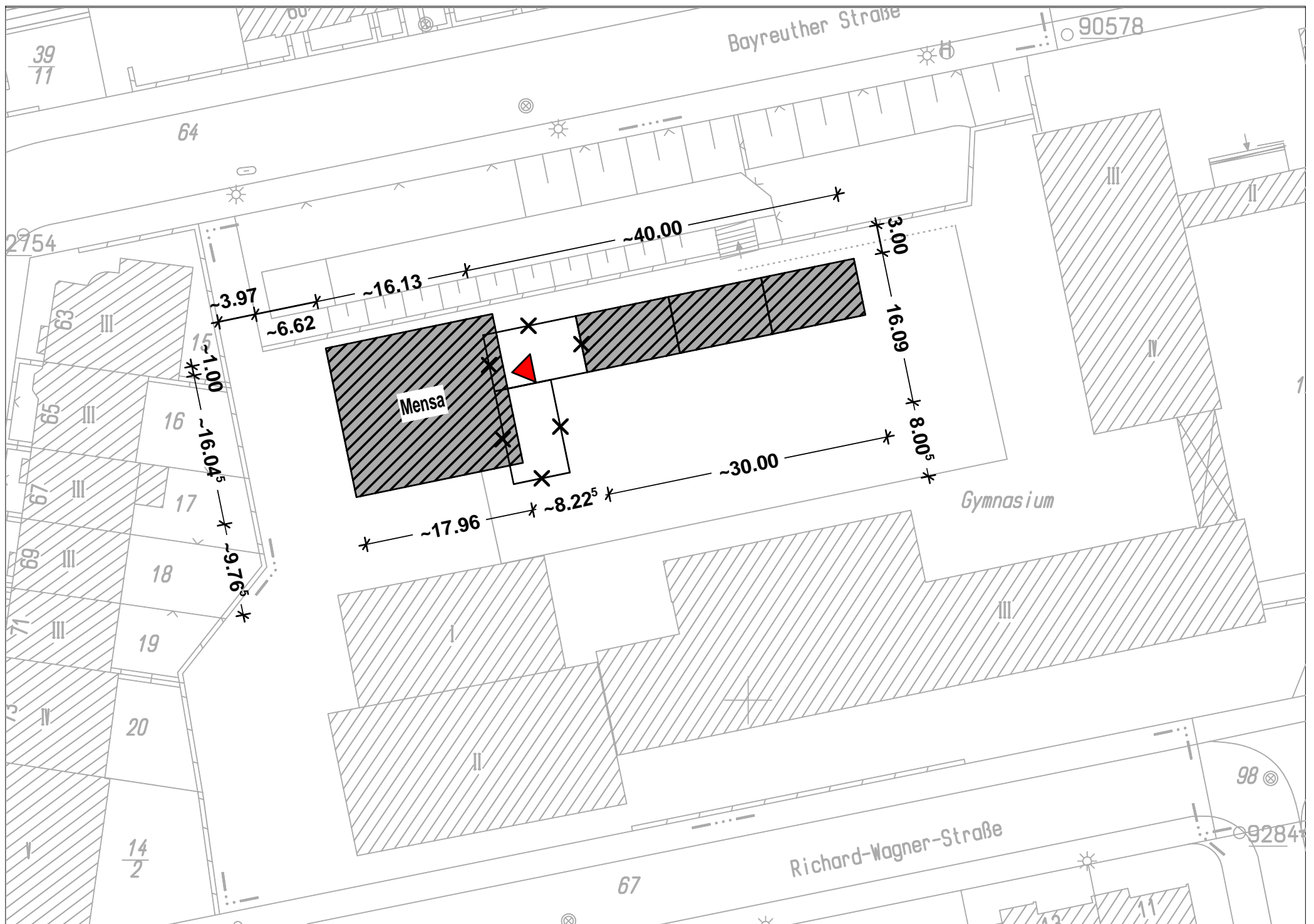
2009-12-14 Lageplan Bayreuther - M 1:500
